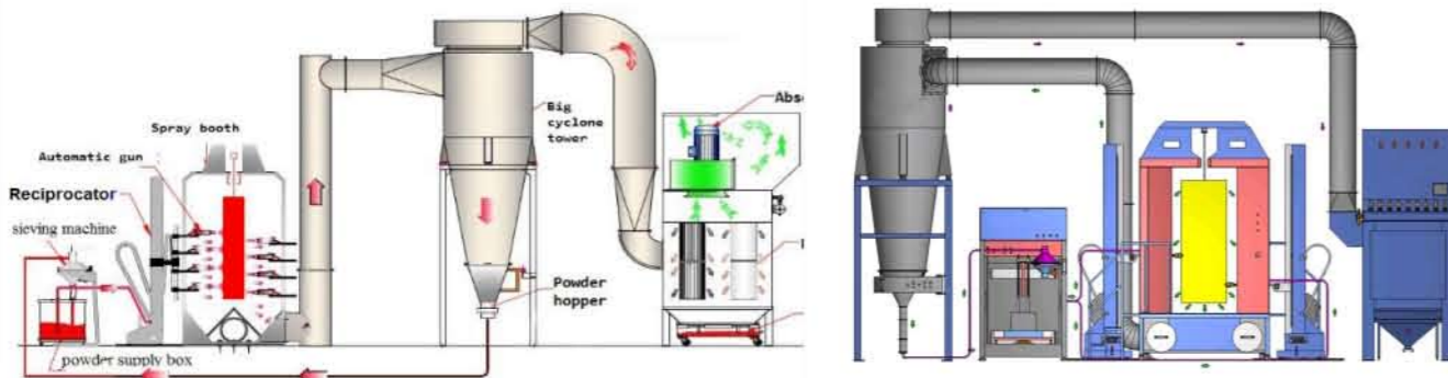
Powder spray booth system -Big cyclone serie
